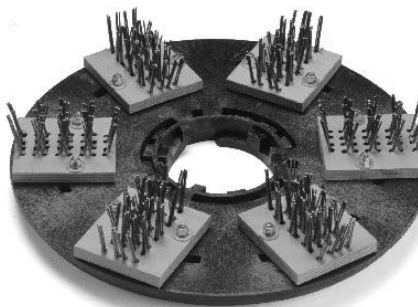
FMA-606207:- 400mm Wire Scarifying Brush
